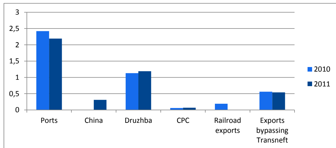
Figure 3-3 Russian crude oil exports in million bbl/dbbl/d (source: CDU-TEK)
