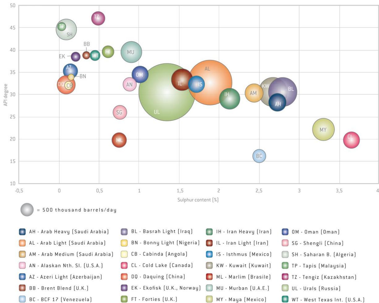
Figure 3-18 Quantities produced globally and properties of main crudes (source: ENI 2012)
