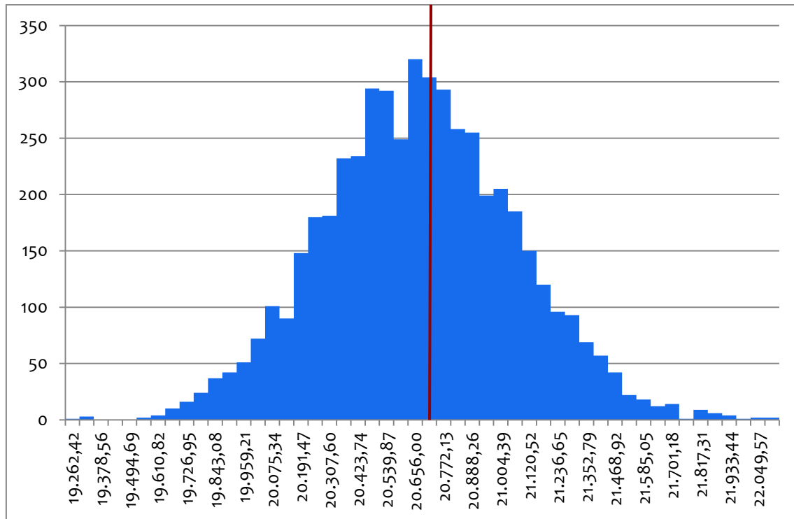
Figure 5-18 Results of the Monte Carlo simulation on the Qatar LNG to South-West EU stream (Red line represents the baseline CI of the stream)
