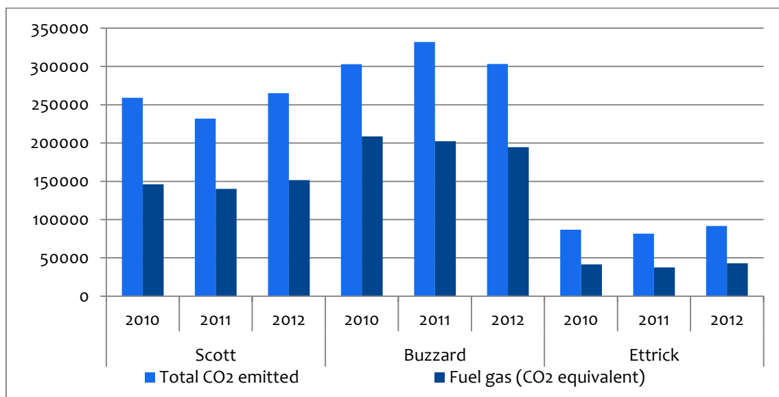
Figure 3-56 Total atmospheric CO 2 emissions and emissions due to consumption of fuel gas for energy production (in tons CO 2 equivalent) for three oil fields (source: NEXEN)
